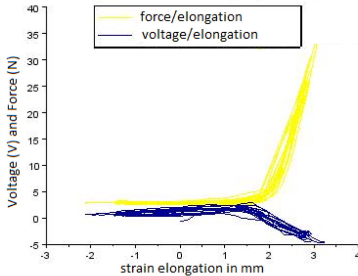
Figure 9: comparison between force/elongation and voltage/ elongation
