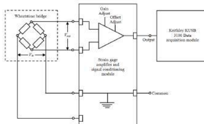
Figure 4: Schematic of the recording devices
