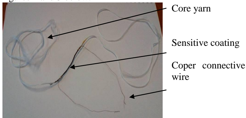
Figure 2: Sensor yarn prototype
