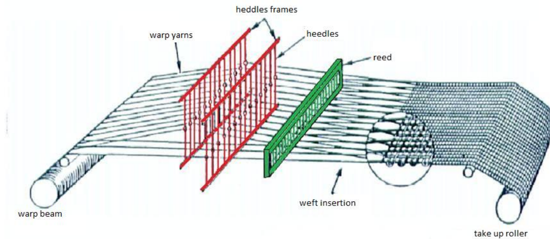
Figure 1: Main weaving loom devices interacting with warp yarns
