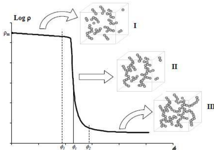
Figure 6: resistivity against conductive particles concentration
