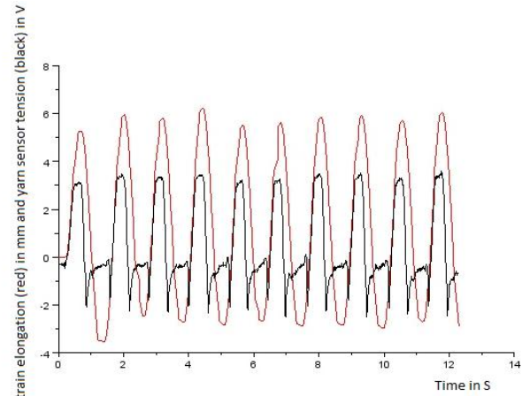
Figure 8: Elongation and voltage versus time
