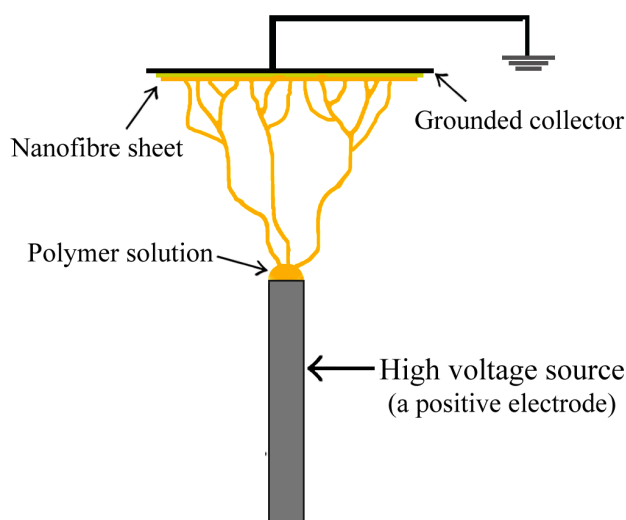
Figure 1: Schematic of a simple electrospinning experiment
